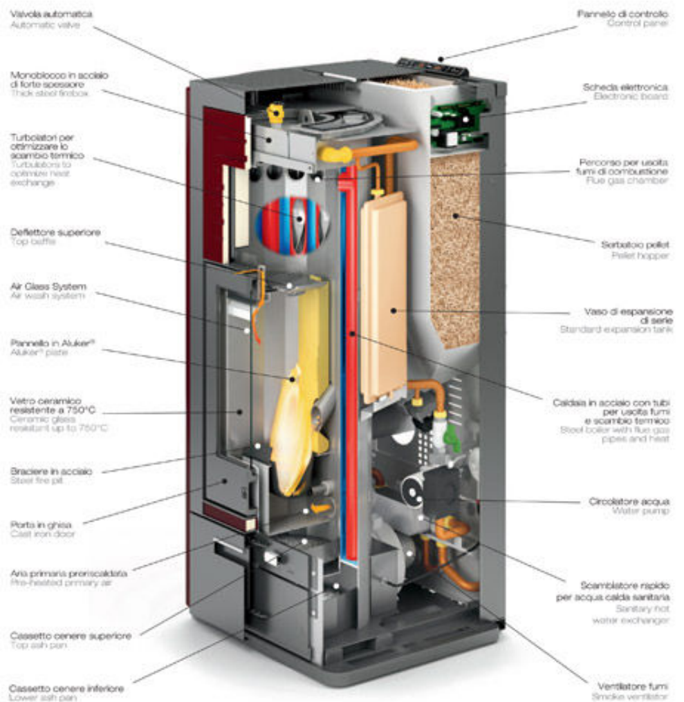
Modello / Model P966 Thermo aca
