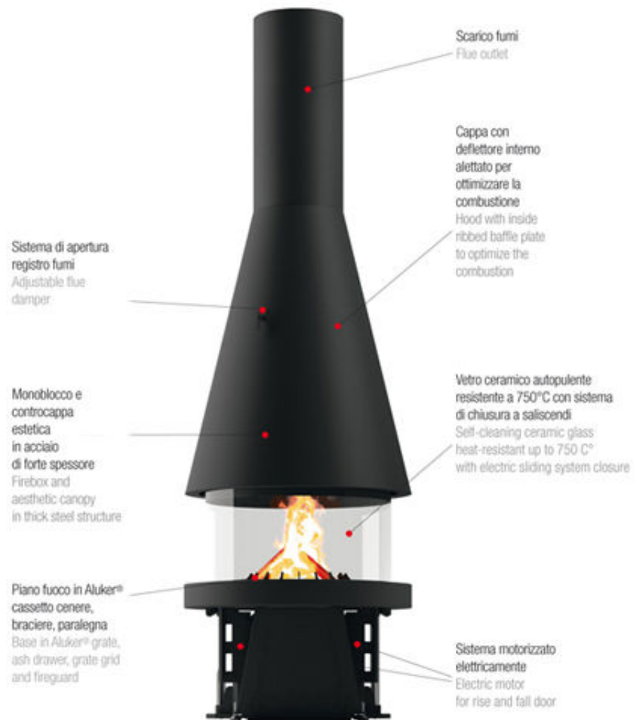
MOD. M360 con cappa conica / with conical hood
